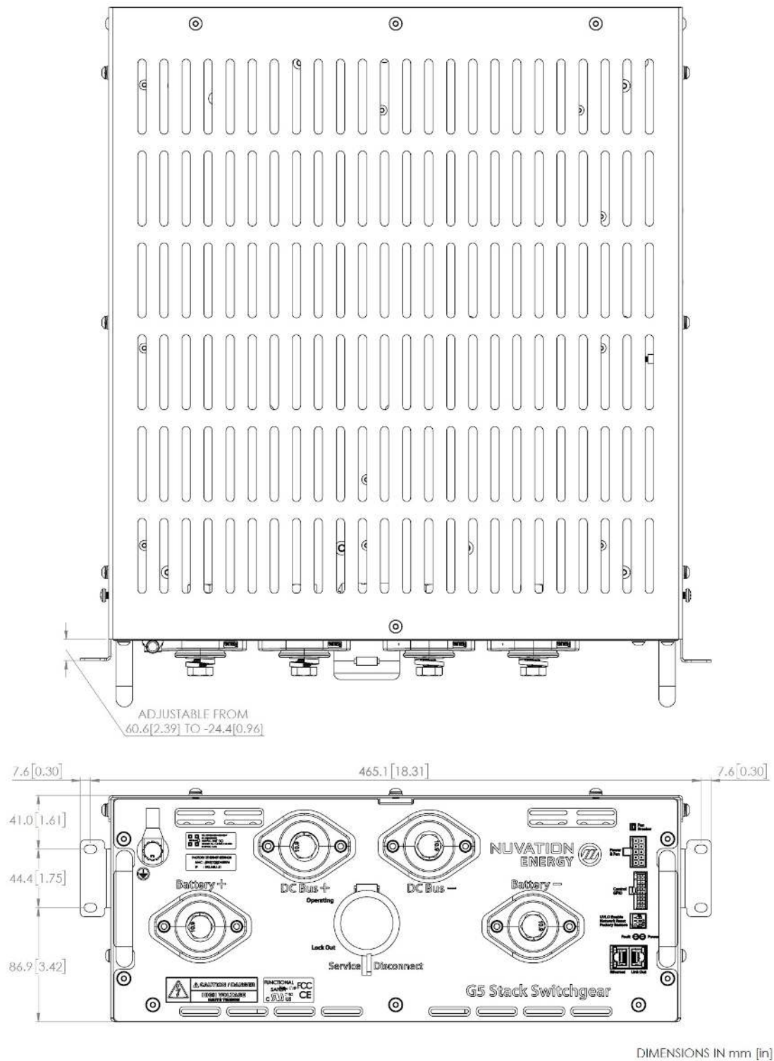
Figure 9. Dimensions, rack-mount, 19", front-securing
